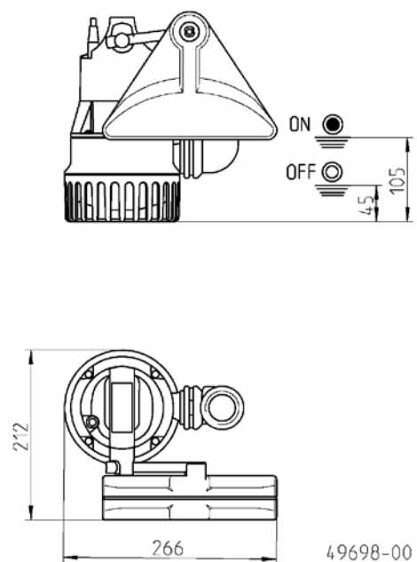
Dimensions and switching points special float (mm)
