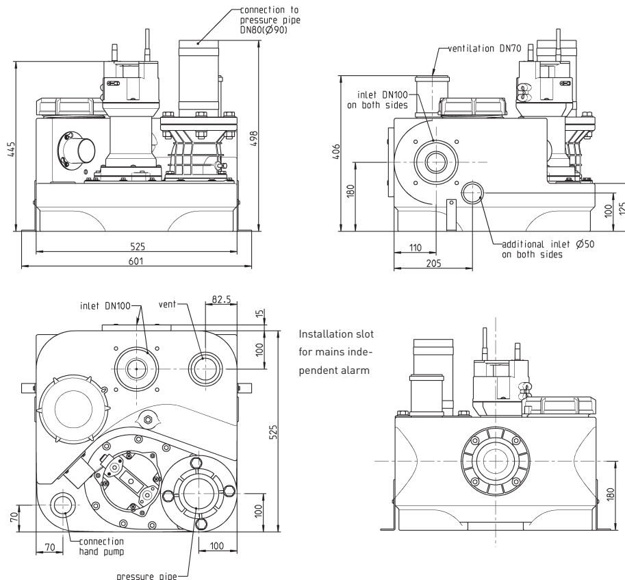
Dimensions with swing-type check valve (mm)
